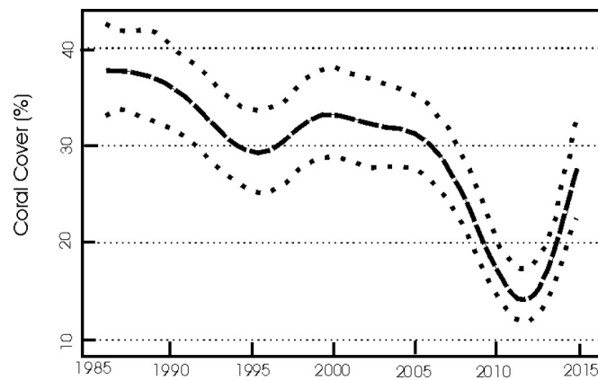
Fig. 8. Mean coral cover for the southern region of the GBR (after AIMS, 2016). Dotted lines represent 95% confidence limits.
