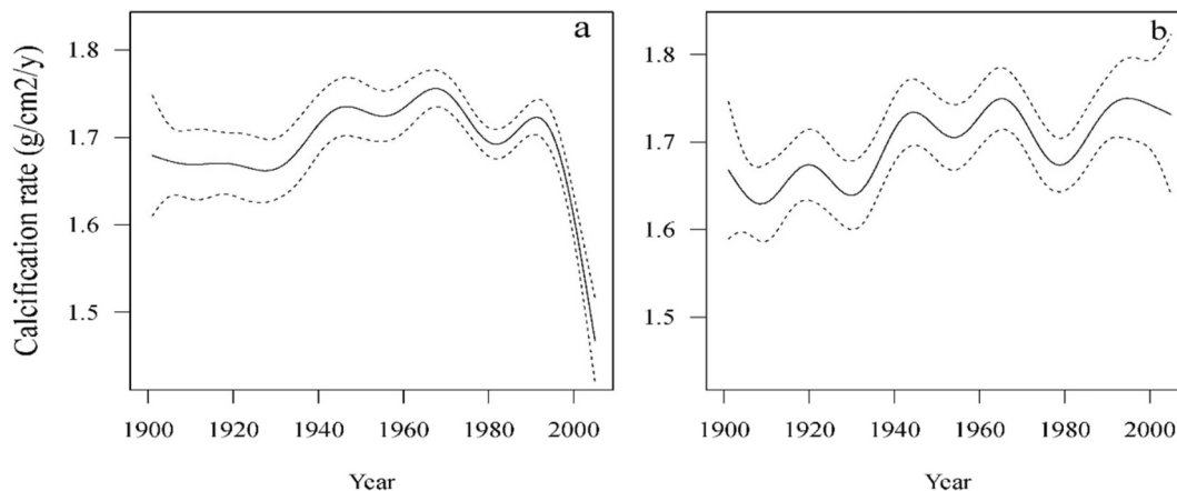
Fig. 6. Coral calcification rate on the GBR for the 20th century. (a) Calculated by De’ath et al. (2009). (b) Reanalysed to account for measurement errors and ontogenetic effects. Dotted lines represent uncertainty margin. (From Ridd et al., 2013).
